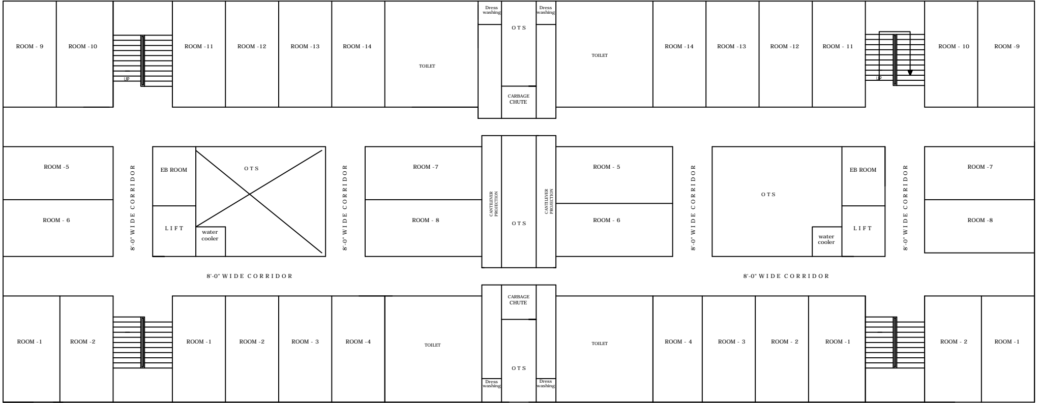
TYPICAL FLOOR PLAN FIRST TO NINTH FLOOR PF HOSTEL"
