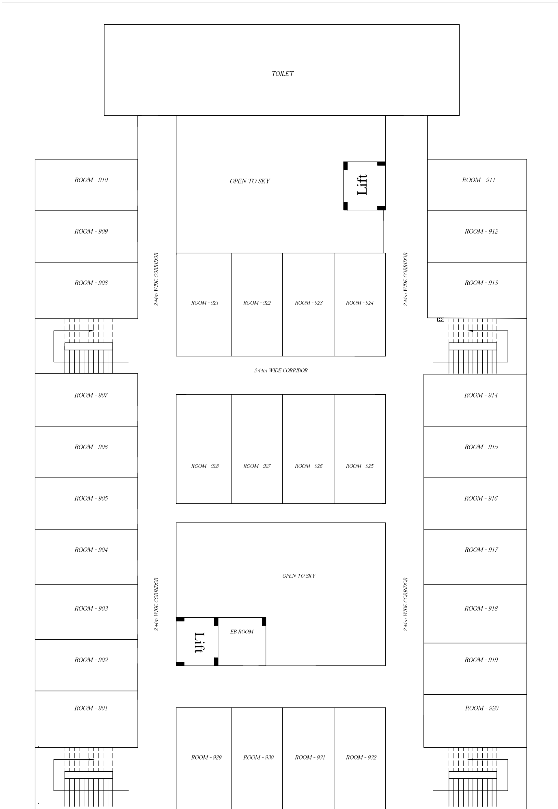
EIGHT FLOOR PLAN KAARI 'H' BLOCK
