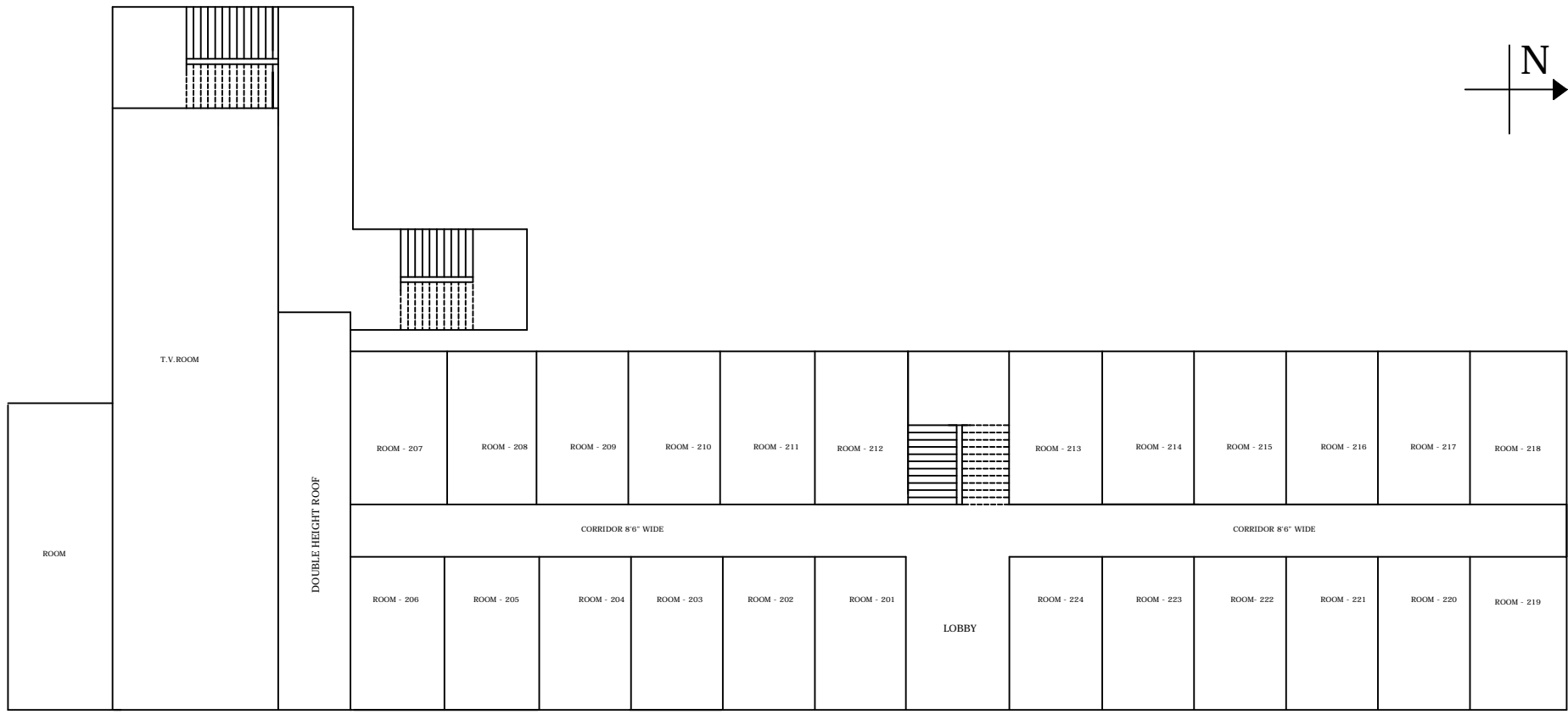
MRS.MEENAKSHI HOSTEL FIRST FLOOR PLAN
