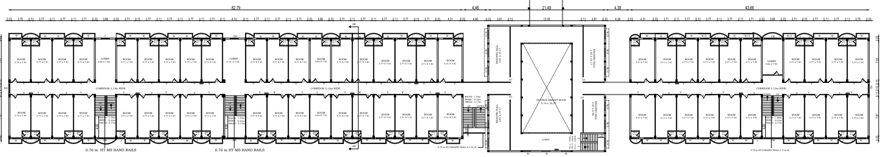
FIRST FLOOR PLAN 'B' BLOCK
