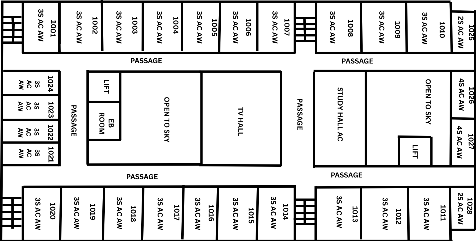
NINTH FLOOR PLAN
