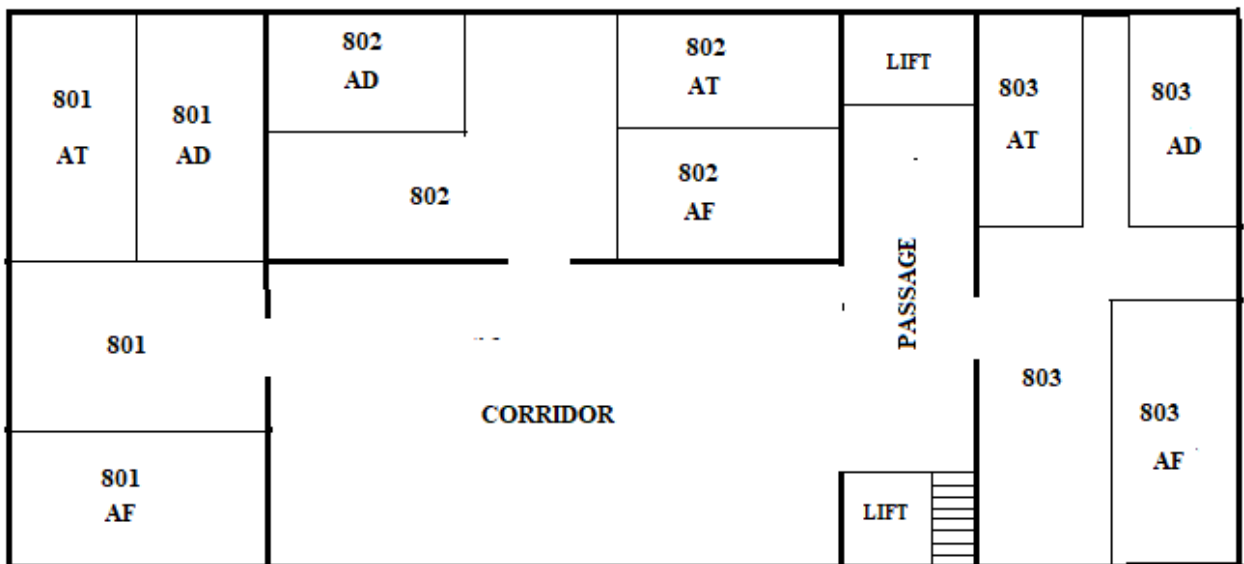
SEVENTH FLOOR PLAN
