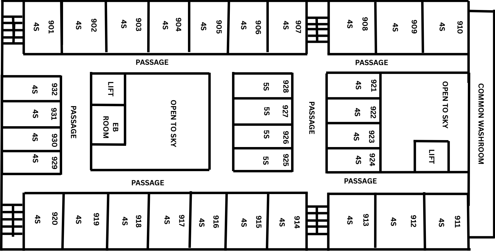
EIGHTH FLOOR PLAN
