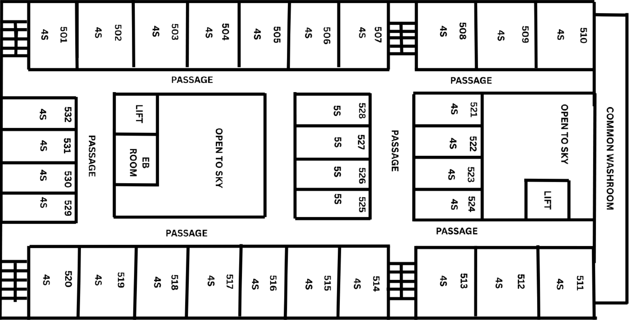
FOURTH FLOOR PLAN
