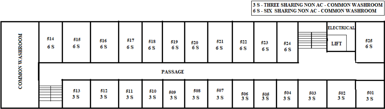
FOURTH FLOOR PLAN
