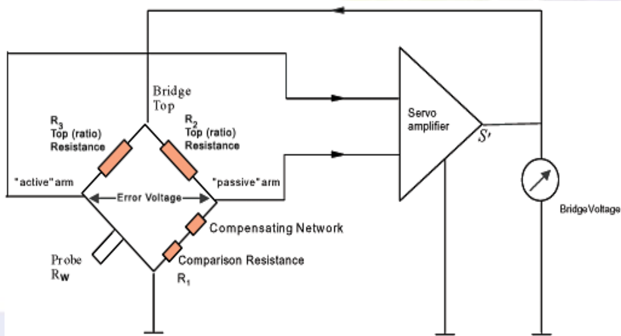
Figure 2. Principal diagram of Constant Temperature Anemometer.
