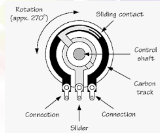
ROTARY POTENTIOMETER
